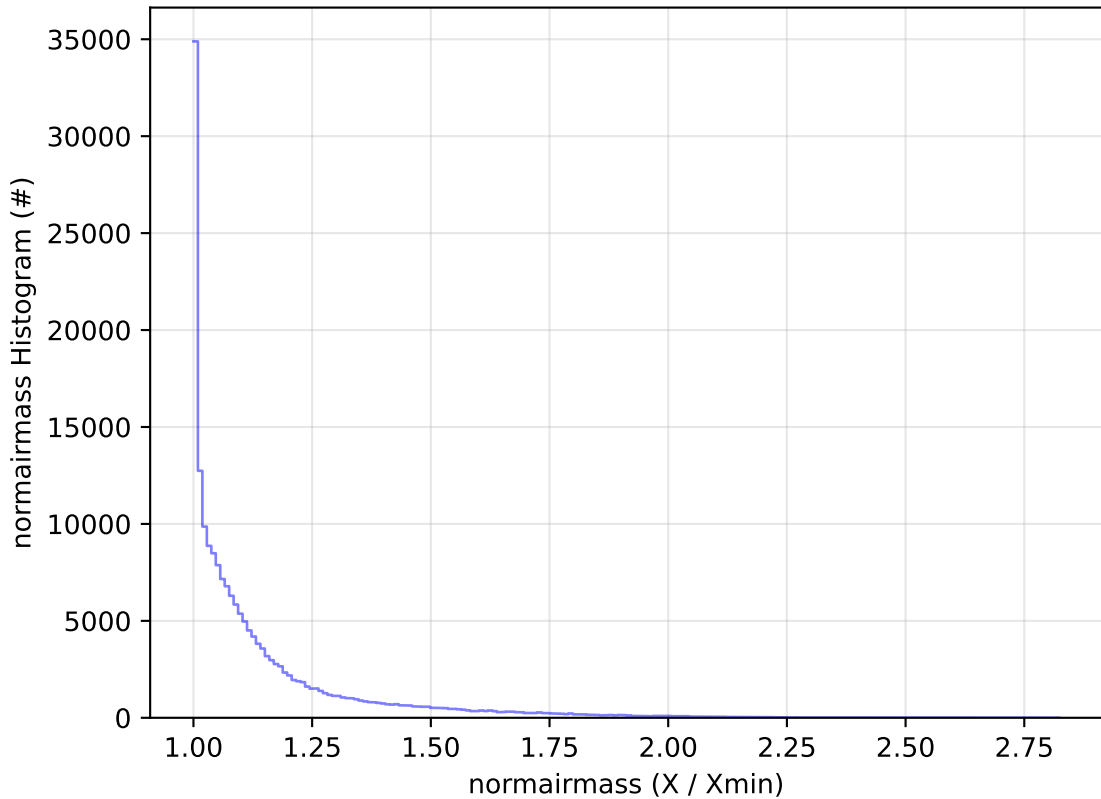
ddf_acor_sf20_lsf0_lsr0_v3.4_10yrs All sky g band: normairmass Histogram
