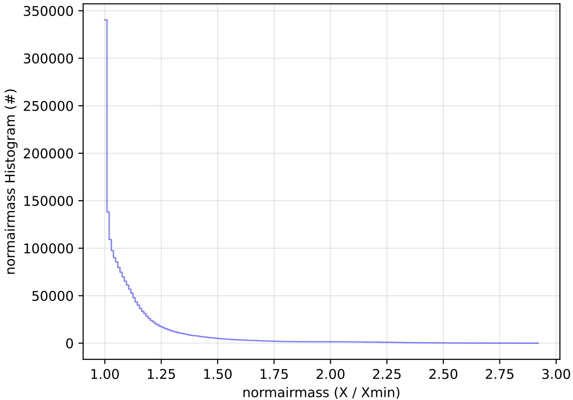
ddf_acor_sf20_lsf0_lsr0_v3.4_10yrs All sky all bands: normairmass Histogram
