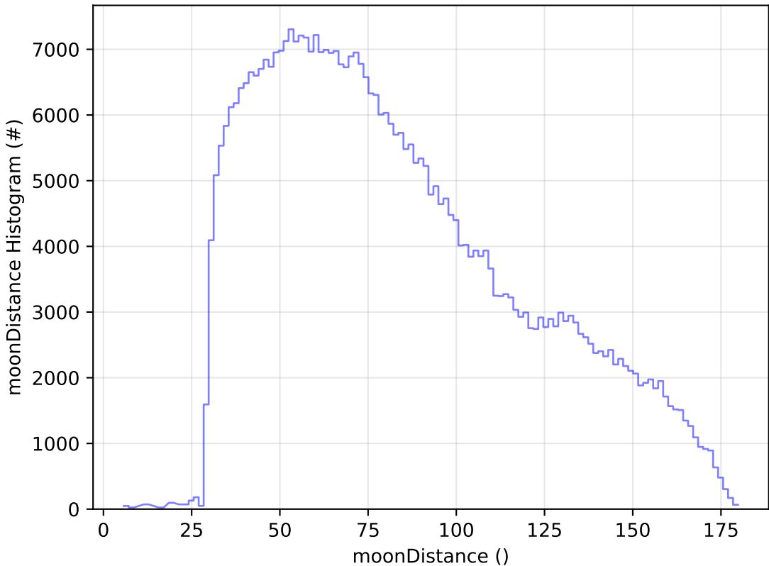
ddf_acor_sf20_lsf0_lsr0_v3.4_10yrs WFD z band: moonDistance Histogram
