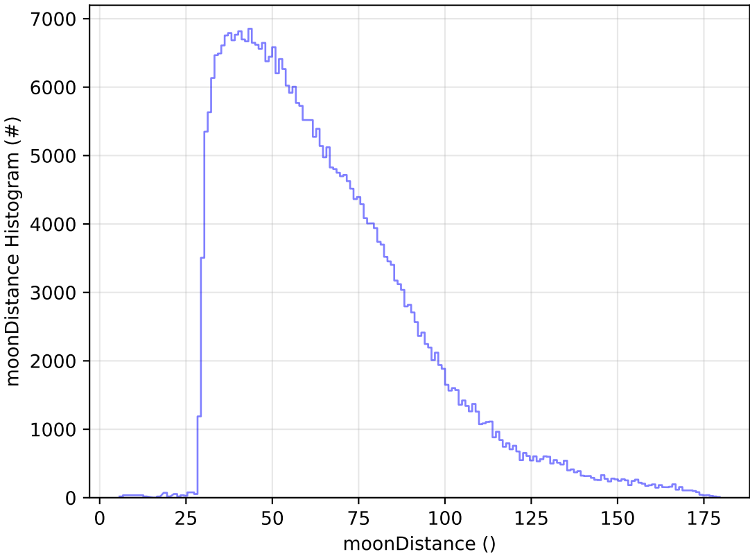
ddf_acor_sf20_lsf0_lsr0_v3.4_10yrs WFD y band: moonDistance Histogram
