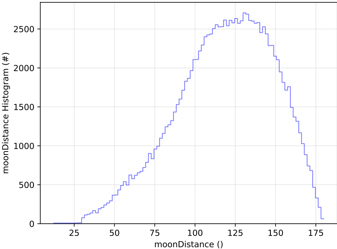
ddf_acor_sf20_lsf0_lsr0_v3.4_10yrs WFD u band: moonDistance Histogram
