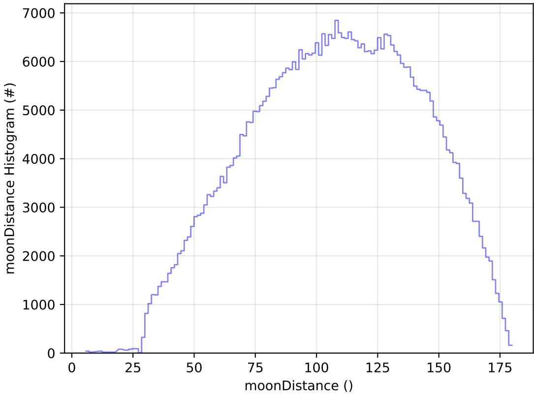
ddf_acor_sf20_lsf0_lsr0_v3.4_10yrs WFD r band: moonDistance Histogram
