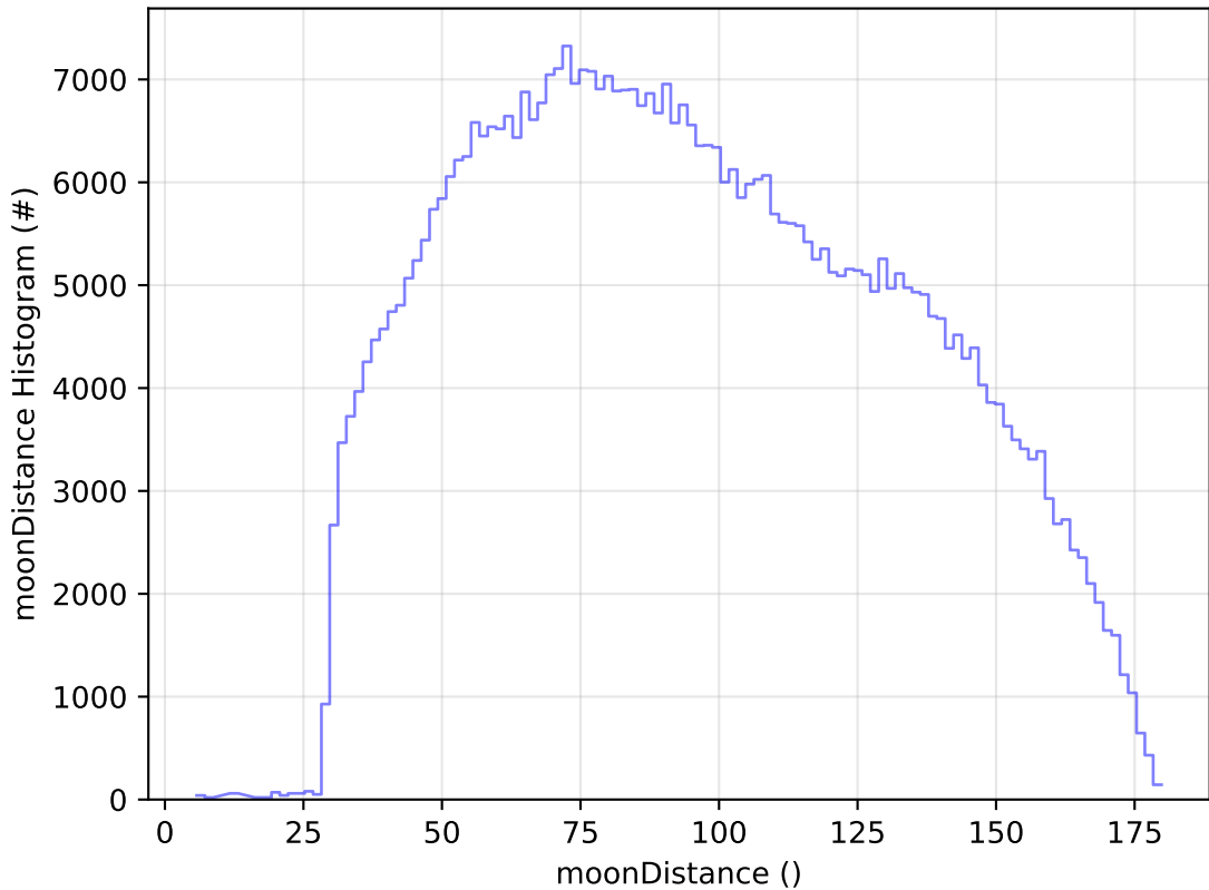
ddf_acor_sf20_lsf0_lsr0_v3.4_10yrs WFD i band: moonDistance Histogram
