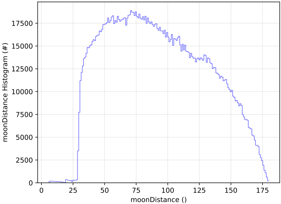
ddf_acor_sf20_lsf0_lsr0_v3.4_10yrs WFD all bands: moonDistance Histogram
