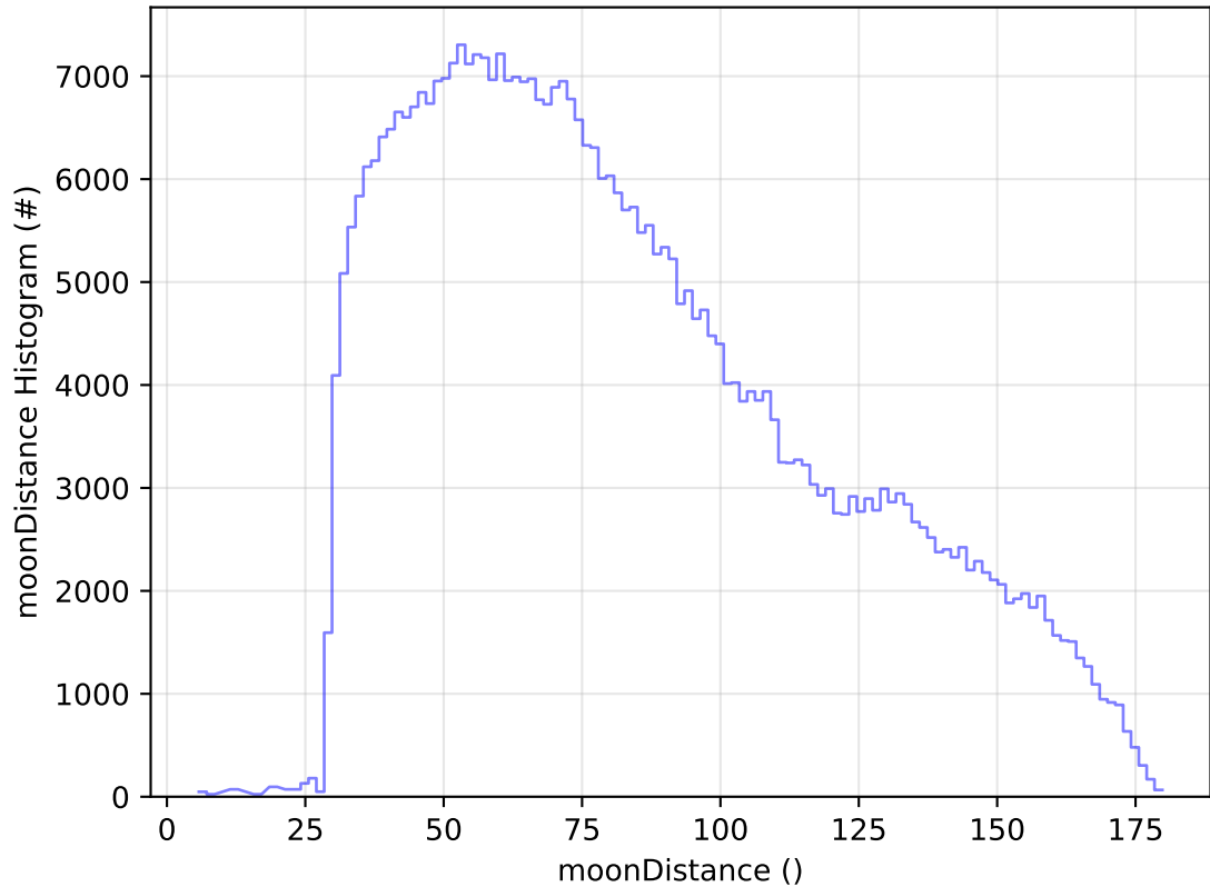
ddf_acor_sf20_lsf0_lsr0_v3.4_10yrs All sky z band: moonDistance Histogram
