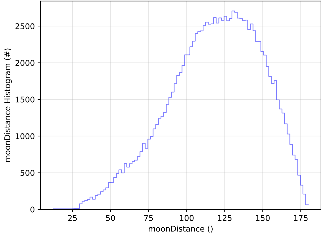
ddf_acor_sf20_lsf0_lsr0_v3.4_10yrs All sky u band: moonDistance Histogram
