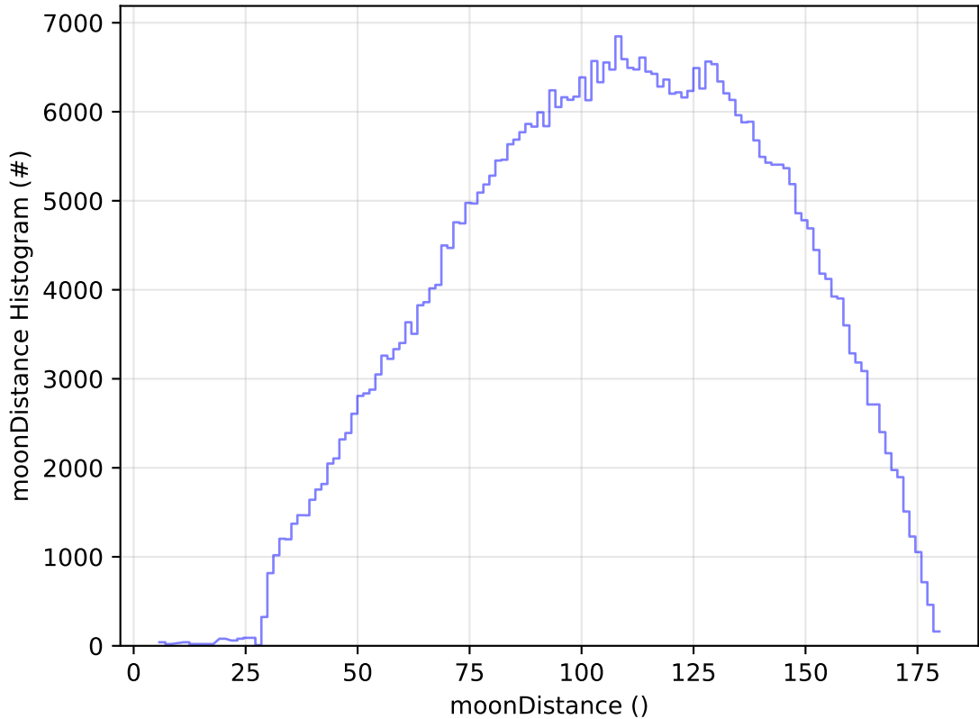
ddf_acor_sf20_lsf0_lsr0_v3.4_10yrs All sky r band: moonDistance Histogram
