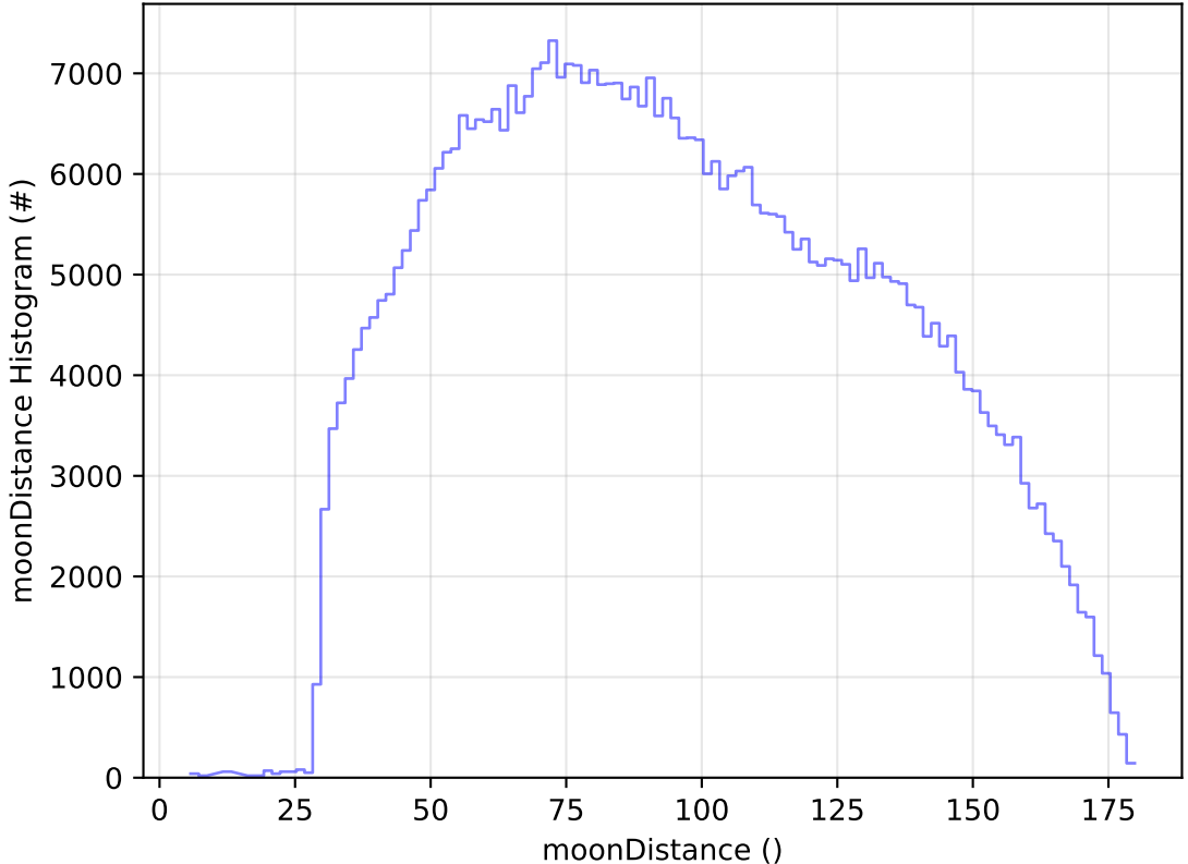
ddf_acor_sf20_lsf0_lsr0_v3.4_10yrs All sky i band: moonDistance Histogram
