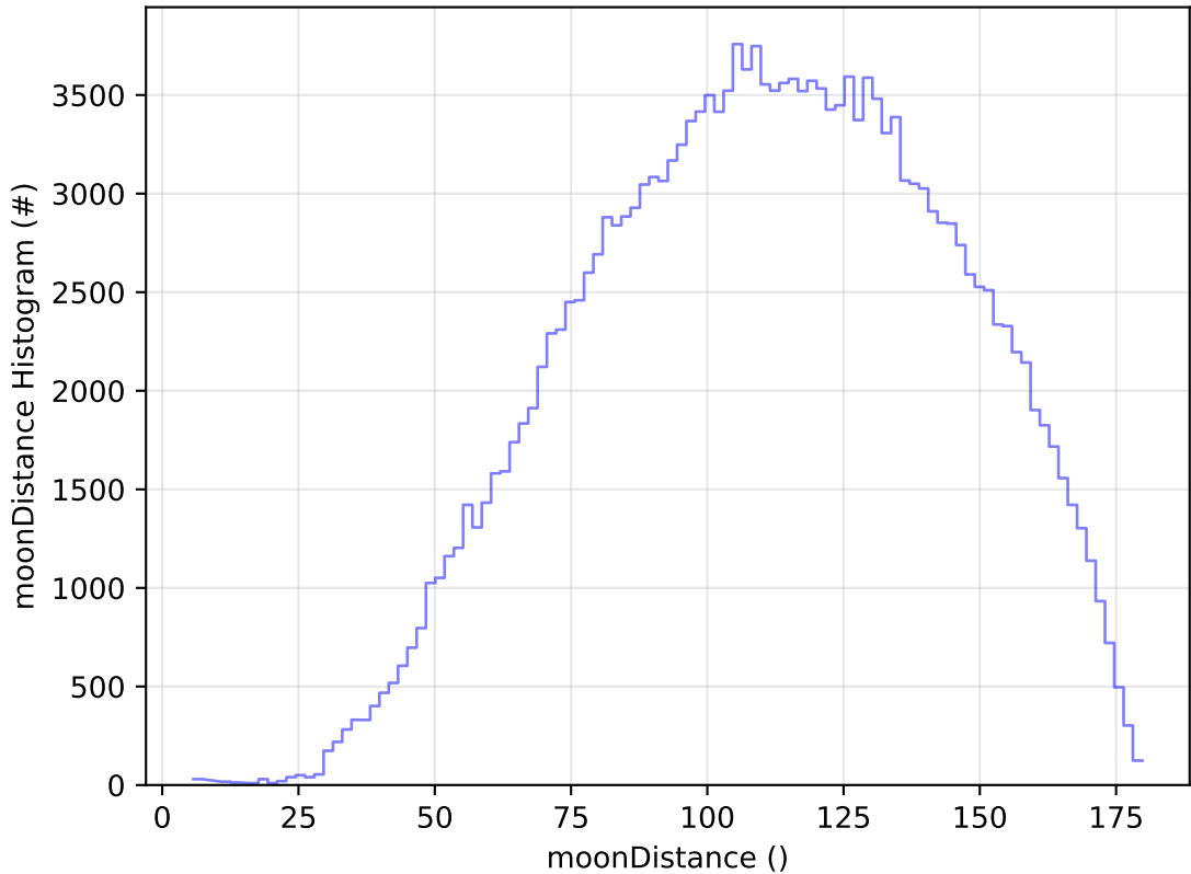
ddf_acor_sf20_lsf0_lsr0_v3.4_10yrs All sky g band: moonDistance Histogram
