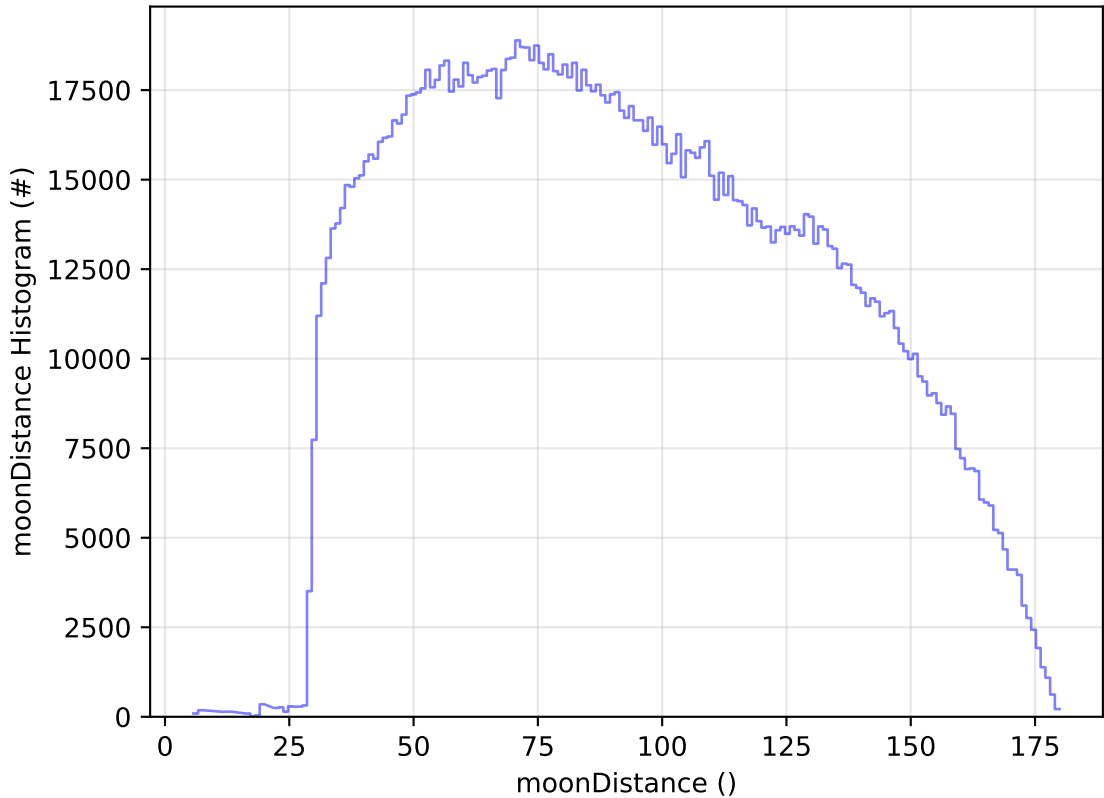
ddf_acor_sf20_lsf0_lsr0_v3.4_10yrs All sky all bands: moonDistance Histogram
