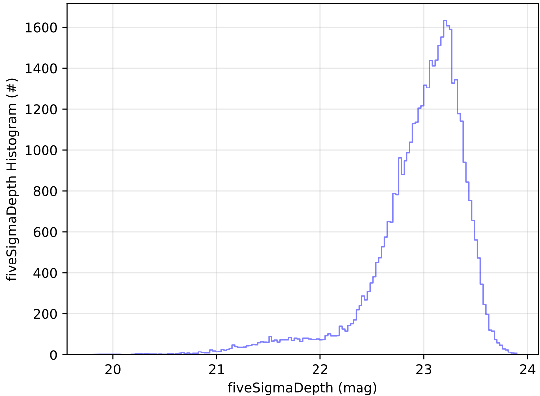
ddf_acor_sf20_lsf0_lsr0_v3.4_10yrs Yr 1 z band: fiveSigmaDepth Histogram
