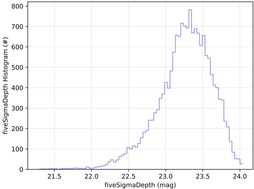
ddf_acor_sf20_lsf0_lsr0_v3.4_10yrs Yr 1 u band: fiveSigmaDepth Histogram
