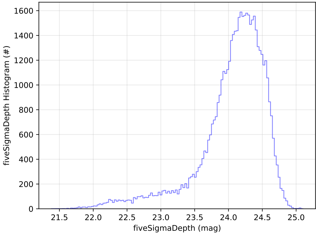
ddf_acor_sf20_lsf0_lsr0_v3.4_10yrs Yr 1 r band: fiveSigmaDepth Histogram
