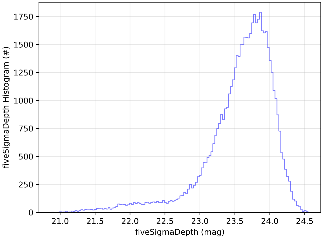
ddf_acor_sf20_lsf0_lsr0_v3.4_10yrs Yr 1 i band: fiveSigmaDepth Histogram
