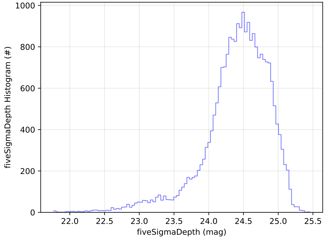
ddf_acor_sf20_lsf0_lsr0_v3.4_10yrs Yr 1 g band: fiveSigmaDepth Histogram
