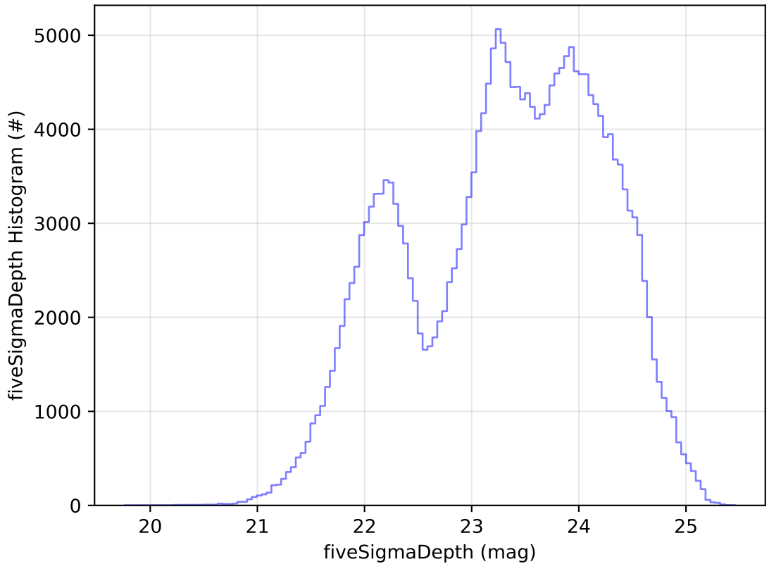
ddf_acor_sf20_ls0_ls0_v3.4_10yrs Yr 1 all bands: fiveSigmaDepth Histogram
