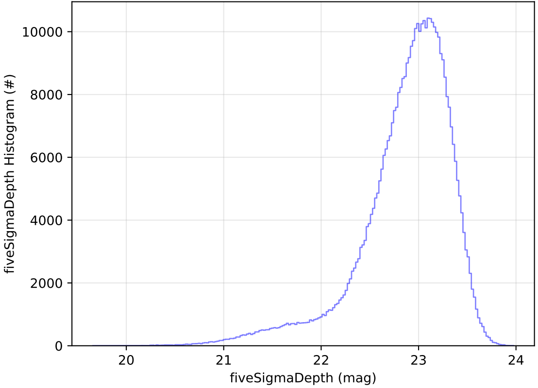
ddf_acor_sf20_lsf0_lsr0_v3.4_10yrs WFD z band: fiveSigmaDepth Histogram
