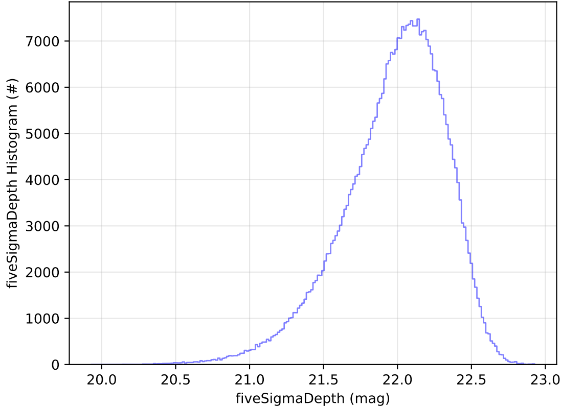
ddf_acor_sf20_lsf0_lsr0_v3.4_10yrs WFD y band: fiveSigmaDepth Histogram
