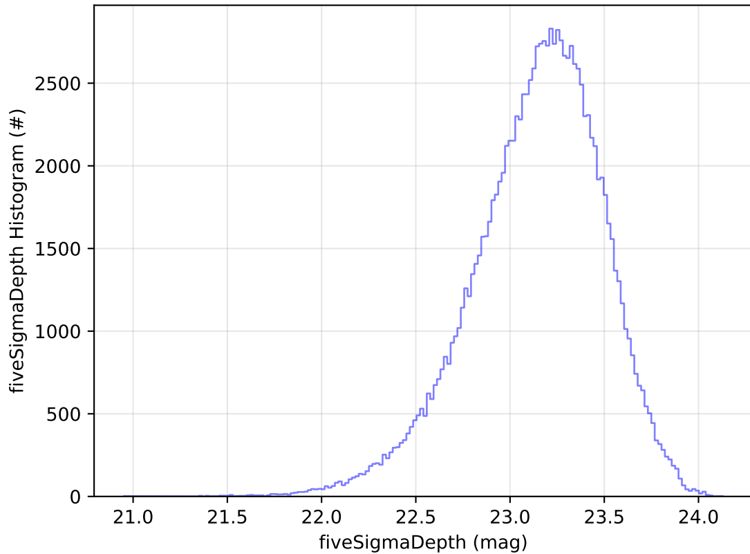
ddf_acor_sf20_lsf0_lsr0_v3.4_10yrs WFD u band: fiveSigmaDepth Histogram
