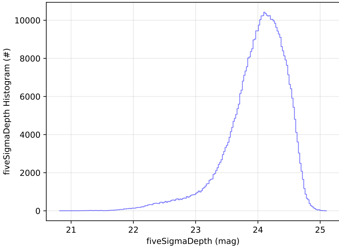
ddf_acor_sf20_lsf0_lsr0_v3.4_10yrs WFD r band: fiveSigmaDepth Histogram
