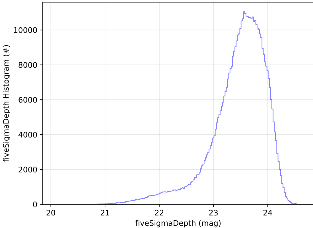
ddf_acor_sf20_lsf0_lsr0_v3.4_10yrs WFD i band: fiveSigmaDepth Histogram
