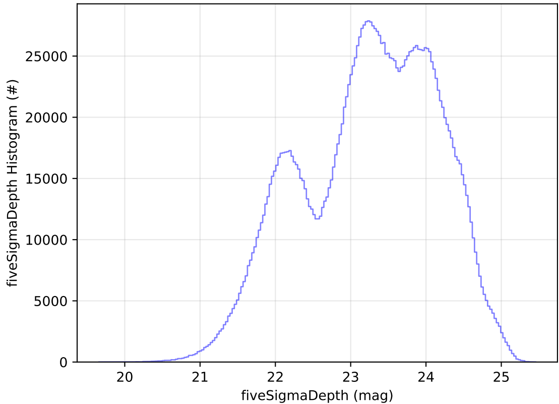
ddf_acor_sf20_lsf0_lsr0_v3.4_10yrs WFD all bands: fiveSigmaDepth Histogram
