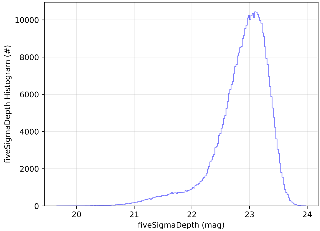
ddf_acor_sf20_lsf0_lsr0_v3.4_10yrs All sky z band: fiveSigmaDepth Histogram
