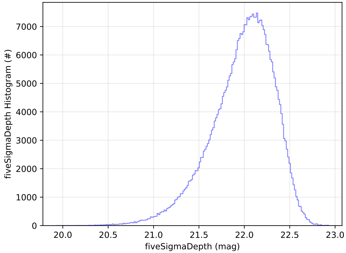
ddf_acor_sf20_lsf0_lsr0_v3.4_10yrs All sky y band: fiveSigmaDepth Histogram
