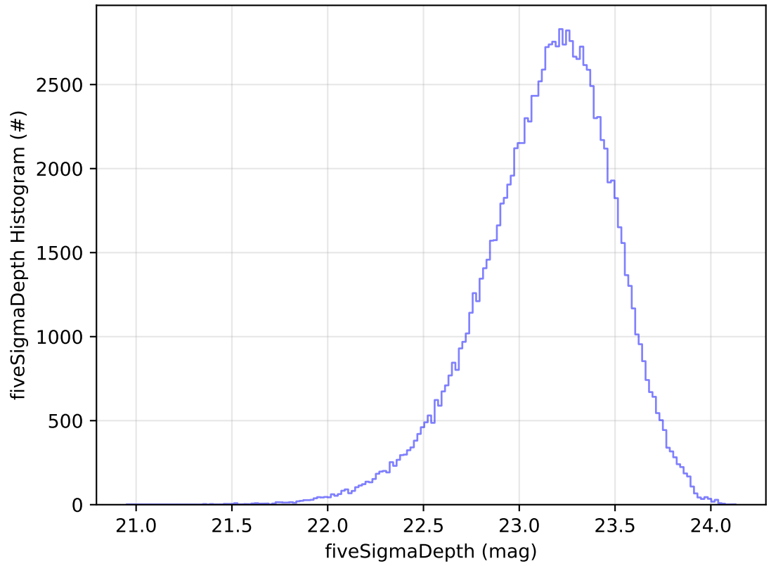
ddf_acor_sf20_lsf0_lsr0_v3.4_10yrs All sky u band: fiveSigmaDepth Histogram
