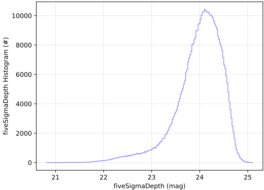
ddf_acor_sf20_lsf0_lsr0_v3.4_10yrs All sky r band: fiveSigmaDepth Histogram
