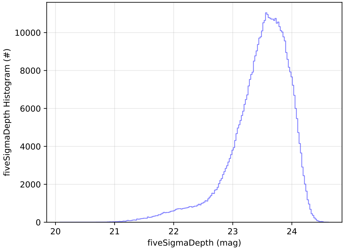
ddf_acor_sf20_lsf0_lsr0_v3.4_10yrs All sky i band: fiveSigmaDepth Histogram
