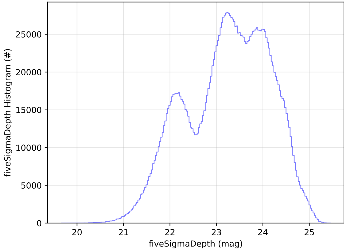
ddf_acor_sf20_lsf0_lsr0_v3.4_10yrs All sky all bands: fiveSigmaDepth Histogram
