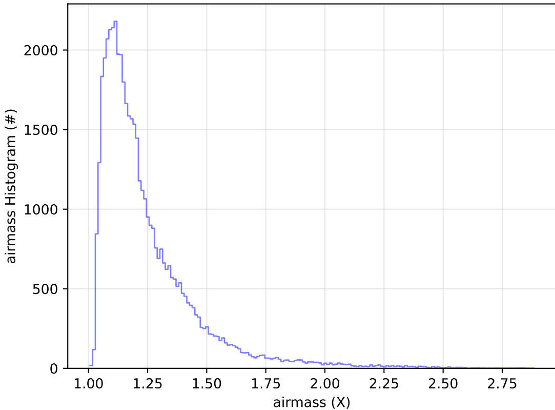
ddf_acor_sf20_lsf0_lsr0_v3.4_10yrs Yr 1 y band: airmass Histogram
