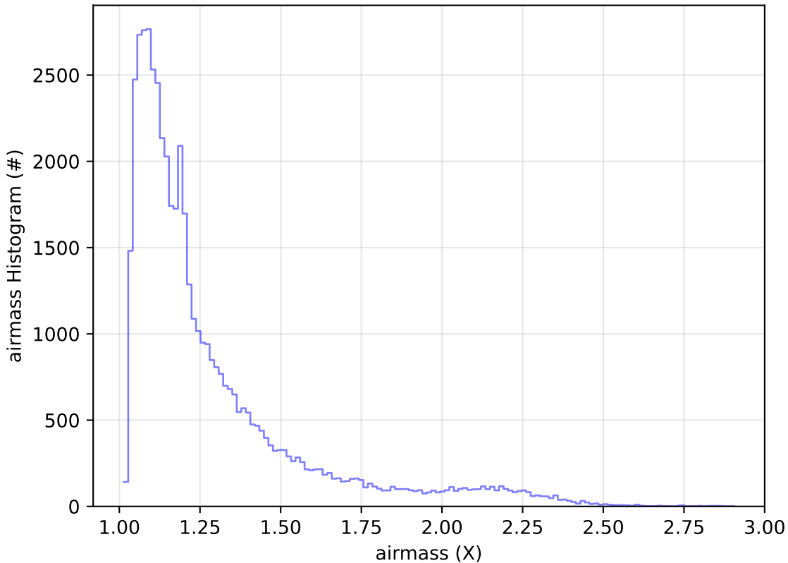
ddf_acor_sf20_lsf0_lsr0_v3.4_10yrs Yr 1 r band: airmass Histogram
