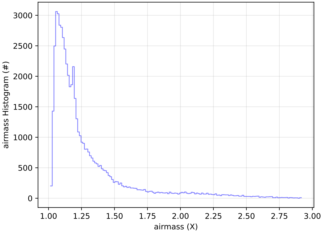
ddf_acor_sf20_lsf0_lsr0_v3.4_10yrs Yr 1 i band: airmass Histogram
