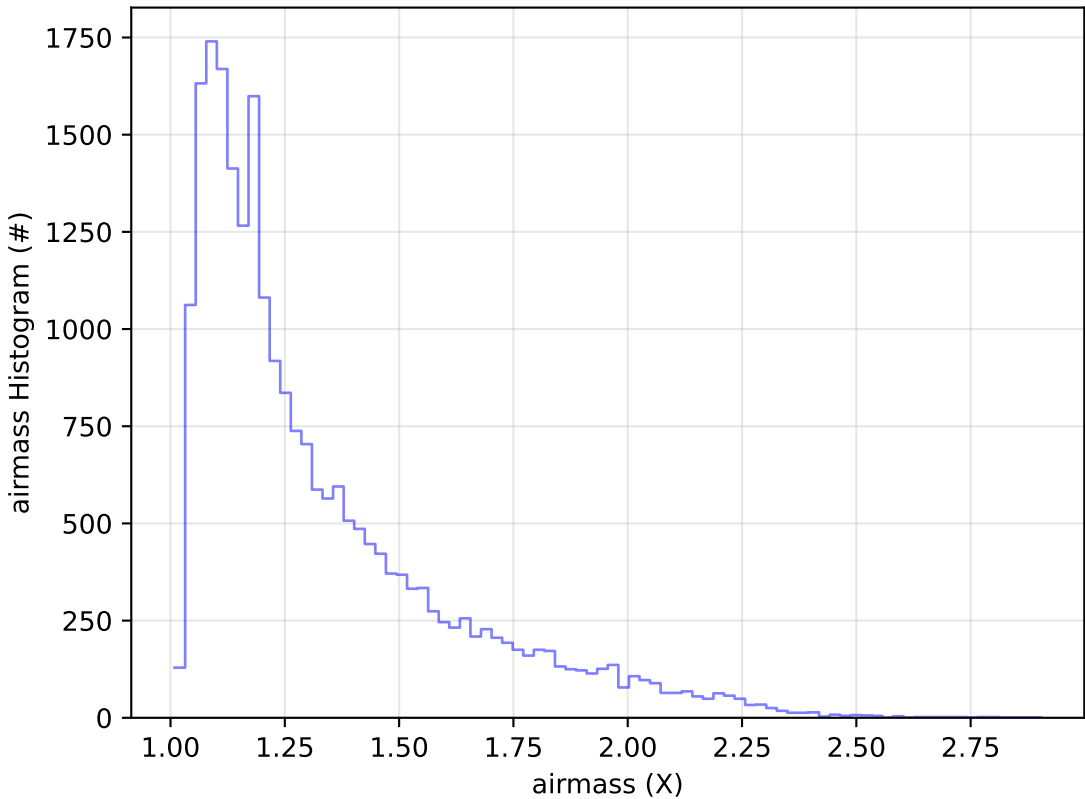
ddf_acor_sf20_lsf0_lsr0_v3.4_10yrs Yr 1 g band: airmass Histogram
