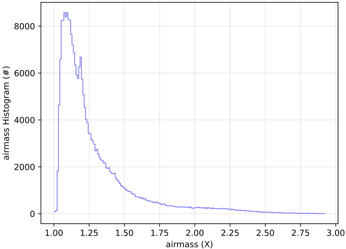
ddf_acor_sf20_lsf0_lsr0_v3.4_10yrs Yr 1 all bands: airmass Histogram
