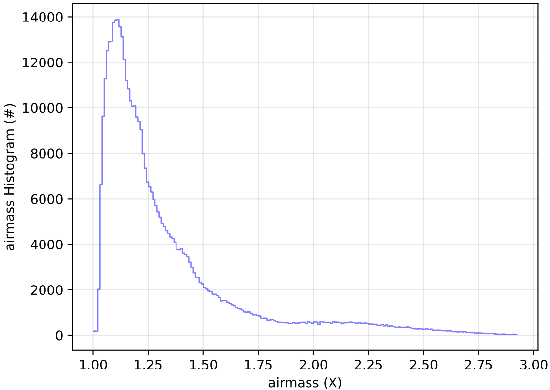
ddf_acor_sf20_lsf0_lsr0_v3.4_10yrs WFD z band: airmass Histogram
