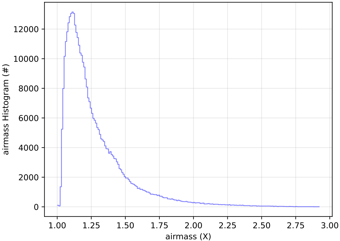
ddf_acor_sf20_lsf0_lsr0_v3.4_10yrs WFD y band: airmass Histogram
