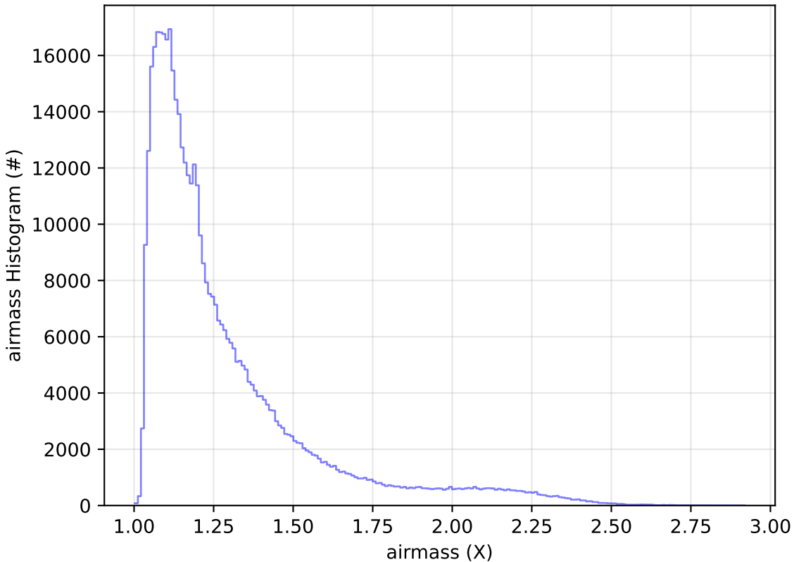
ddf_acor_sf20_lsf0_lsr0_v3.4_10yrs WFD r band: airmass Histogram
