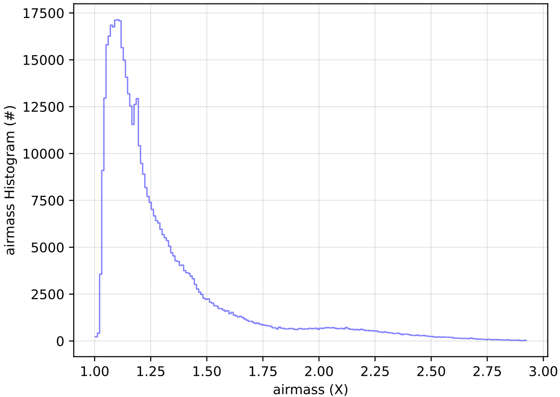
ddf_acor_sf20_lsf0_lsr0_v3.4_10yrs WFD i band: airmass Histogram
