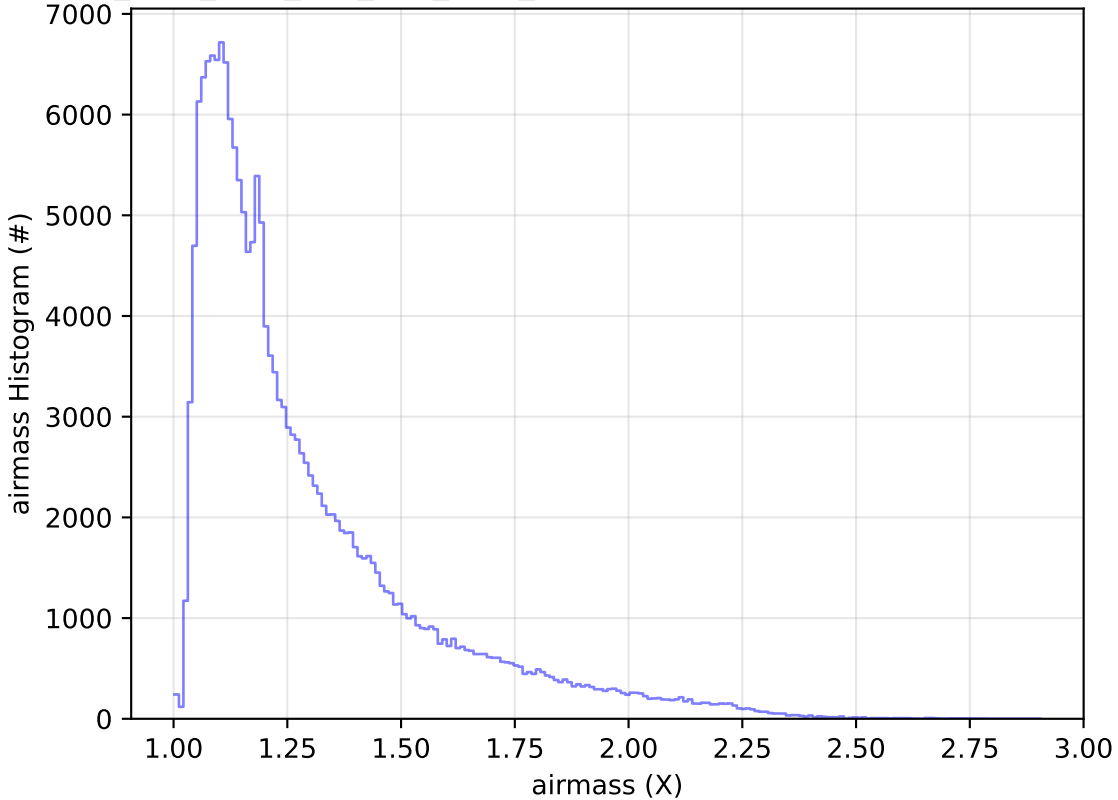
ddf_acor_sf20_lsf0_lsr0_v3.4_10yrs WFD g band: airmass Histogram
