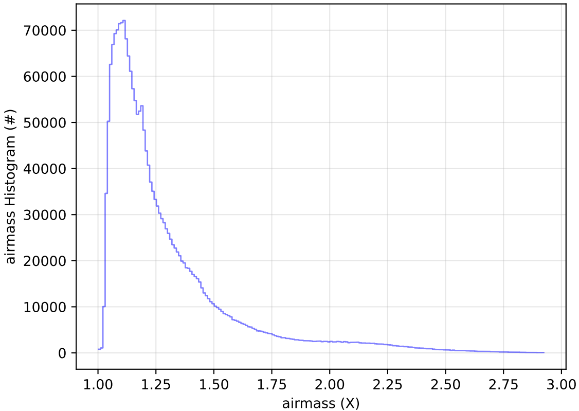
ddf_acor_sf20_lsf0_lsr0_v3.4_10yrs WFD all bands: airmass Histogram
