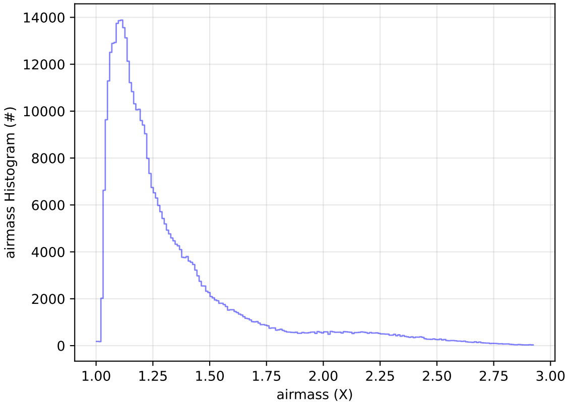
ddf_acor_sf20_lsf0_lsr0_v3.4_10yrs All sky z band: airmass Histogram
