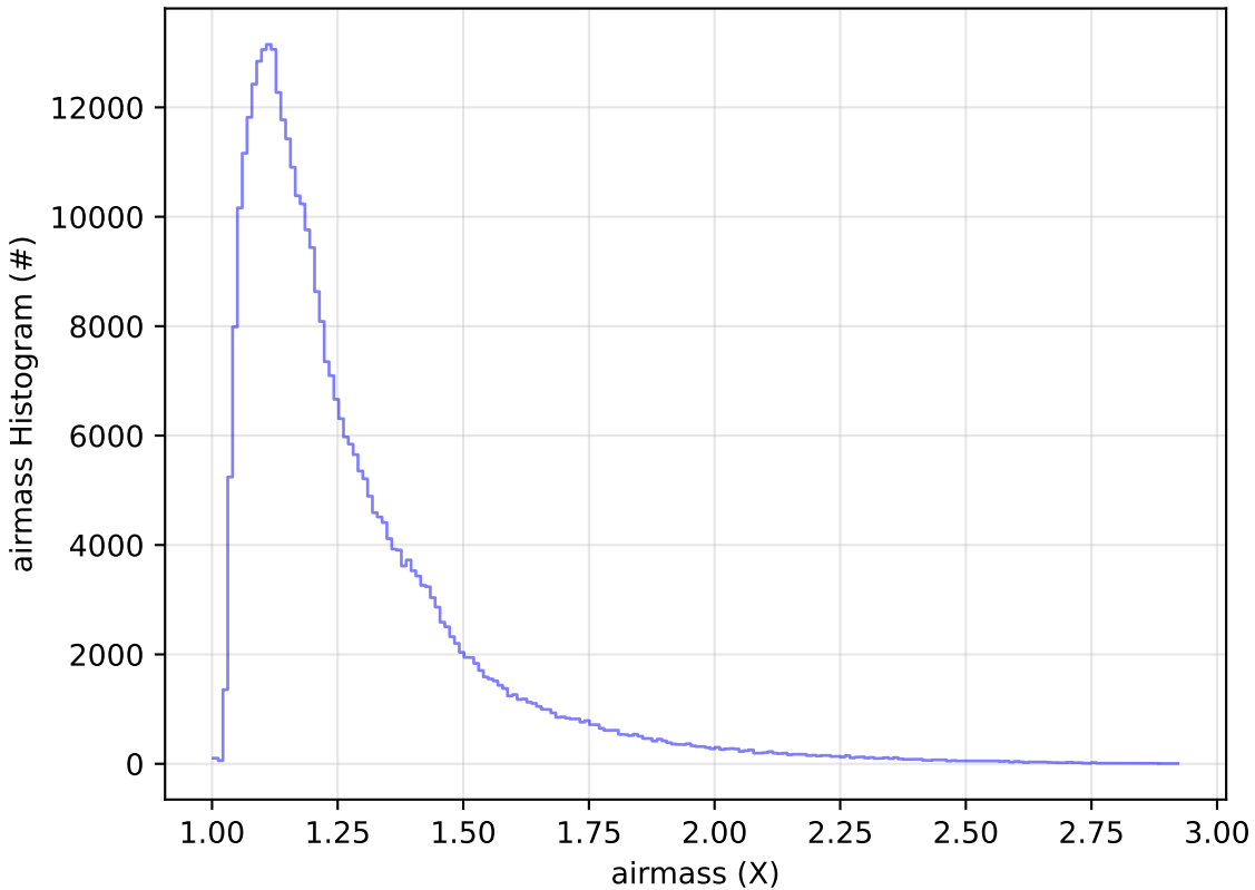
ddf_acor_sf20_lsf0_lsr0_v3.4_10yrs All sky y band: airmass Histogram
