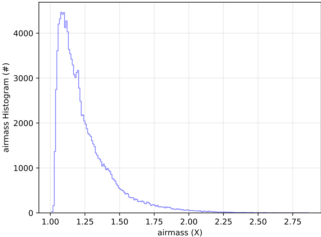
ddf_acor_sf20_ls0_lsr0_v3.4_10yrs All sky u band: airmass Histogram
