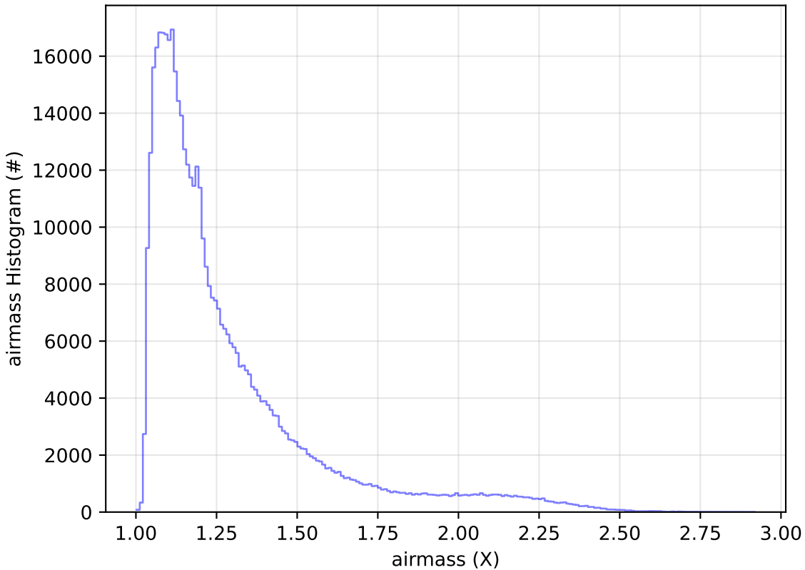
ddf_acor_sf20_lsf0_lsr0_v3.4_10yrs All sky r band: airmass Histogram
