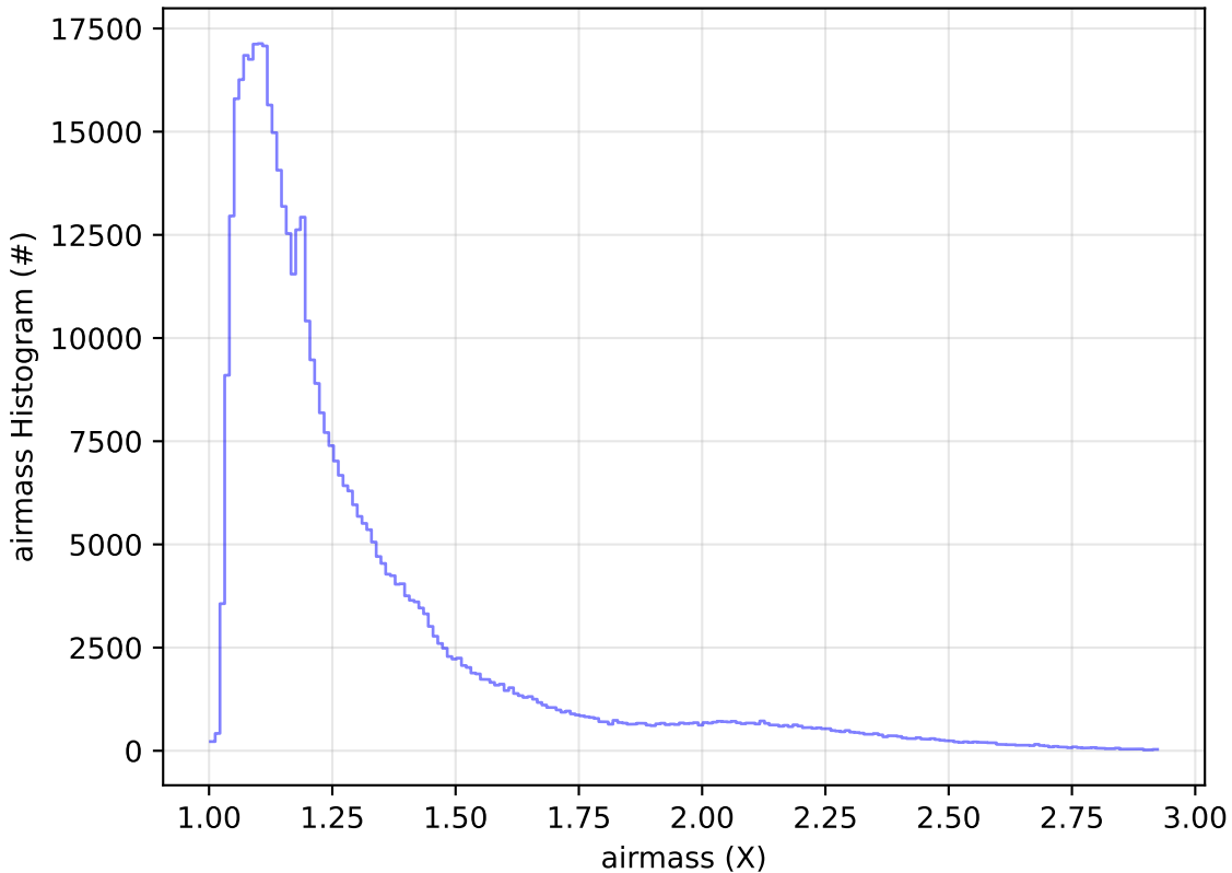
ddf_acor_sf20_ls0_lsr0_v3.4_10yrs All sky i band: airmass Histogram
