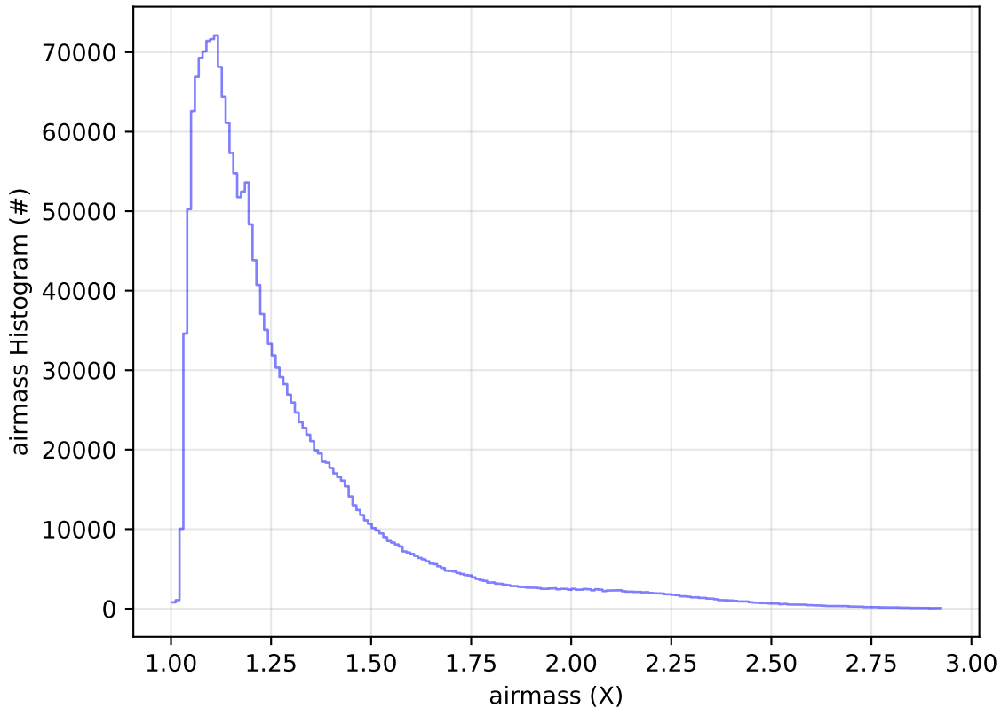
ddf_acor_sf20_lsf0_lsr0_v3.4_10yrs All sky all bands: airmass Histogram
