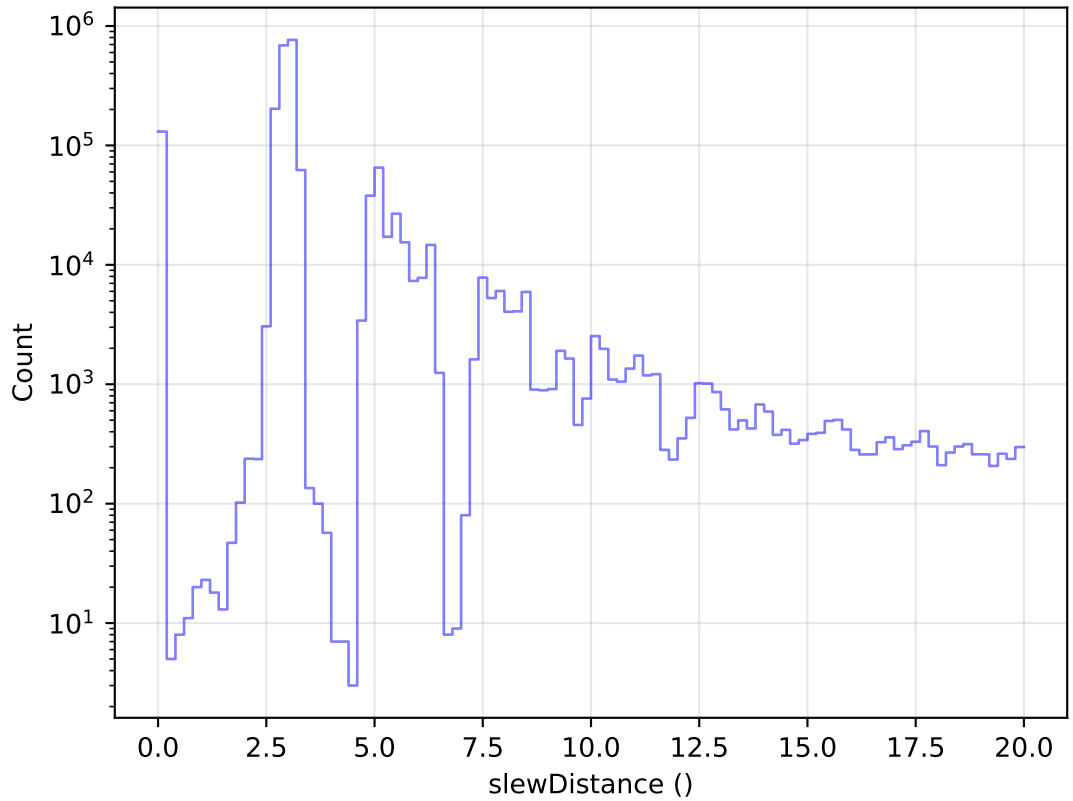
ddf_acor_sf20_lsf0_lsr0_v3.4_10yrs All visits: Zoom Slew Distance Histogram
